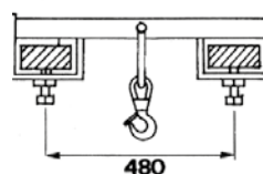
MINF-2 / MINF-3 Inforcabile tramite 2 forche Used with two forks
