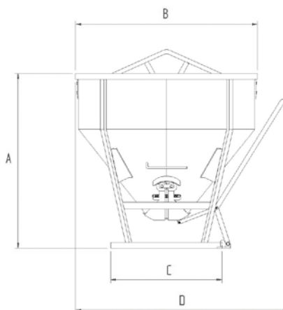
Benna conica a scarico centrale Conical bucket with central unloading
